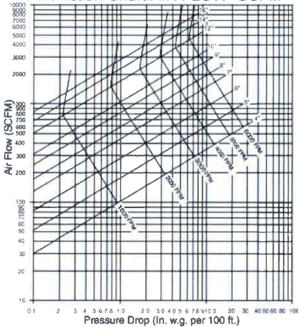
Air Friction Chart AIR FLOW "SCFM"
